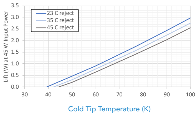
Nominal Performance at Different Reject Temperatures
